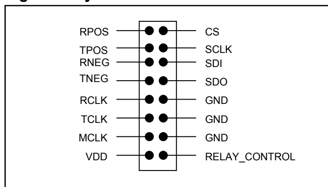
Figure 3. System Connector
