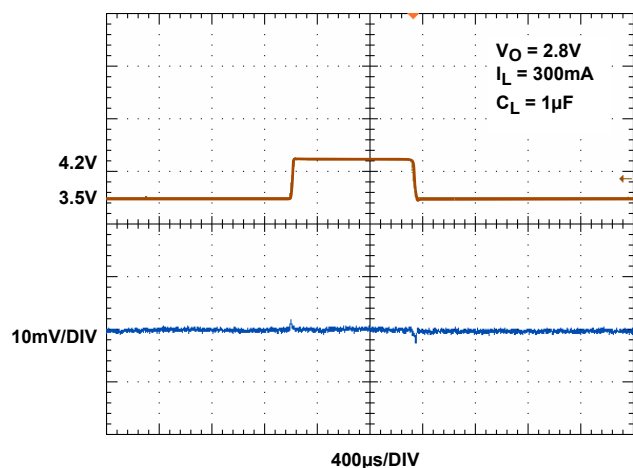
FIGURE 15. LINE TRANSIENT RESPONSE, 2.8V OUTPUT
