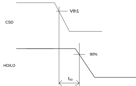
Figure 2: CSD to Shutdown Waveform Definitions
