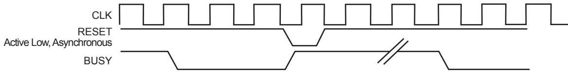
Figure 2-44 • Reset Timing Diagram
