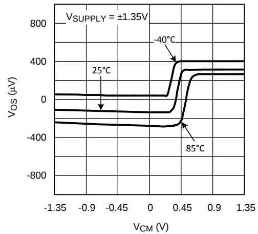
Figure 2. V_{OS} vs. V_{CM}
