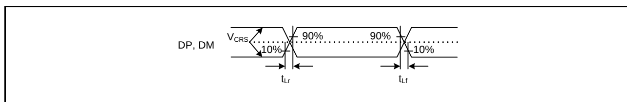
Figure 5.38 DP and DM Output Timing (Full-Speed)
