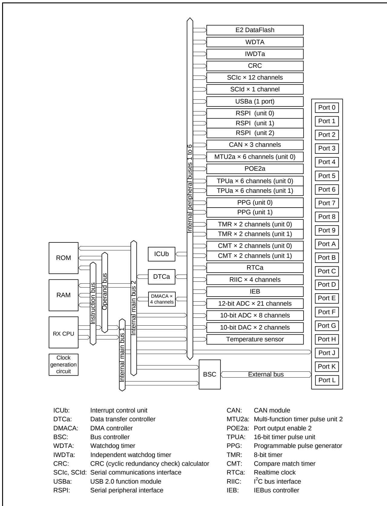
Figure 1.2 Block Diagram
