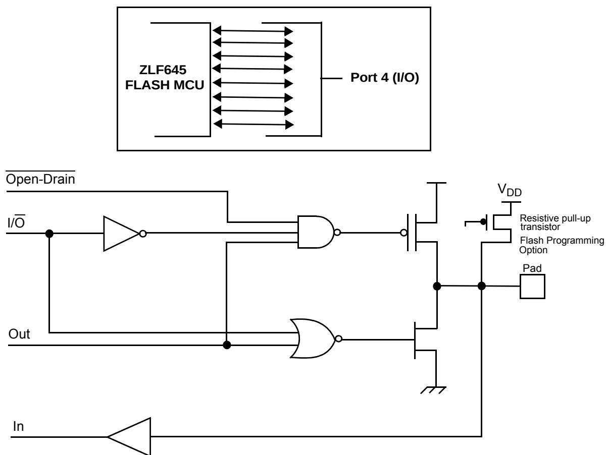
Figure 11. Port 4 Configuration
