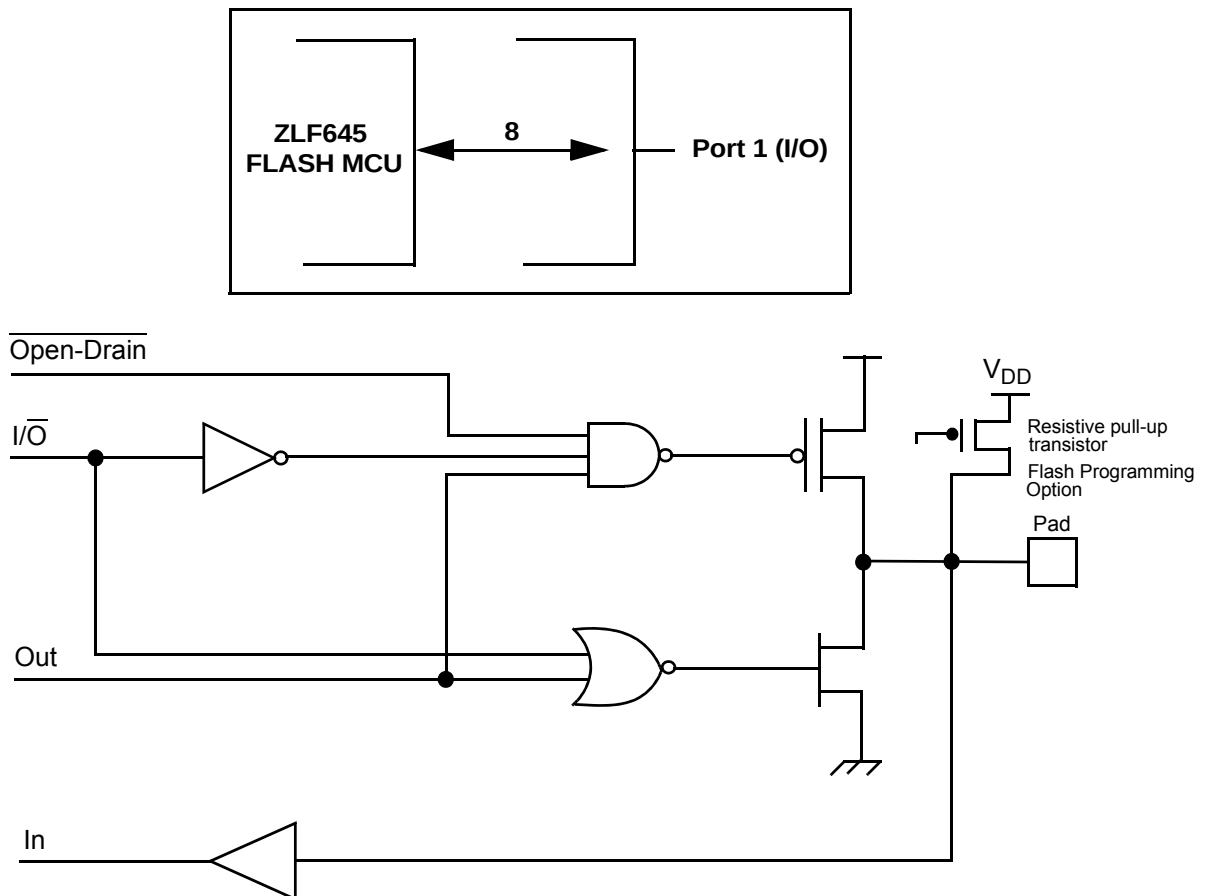
Figure 7. Port 1 Configuration
