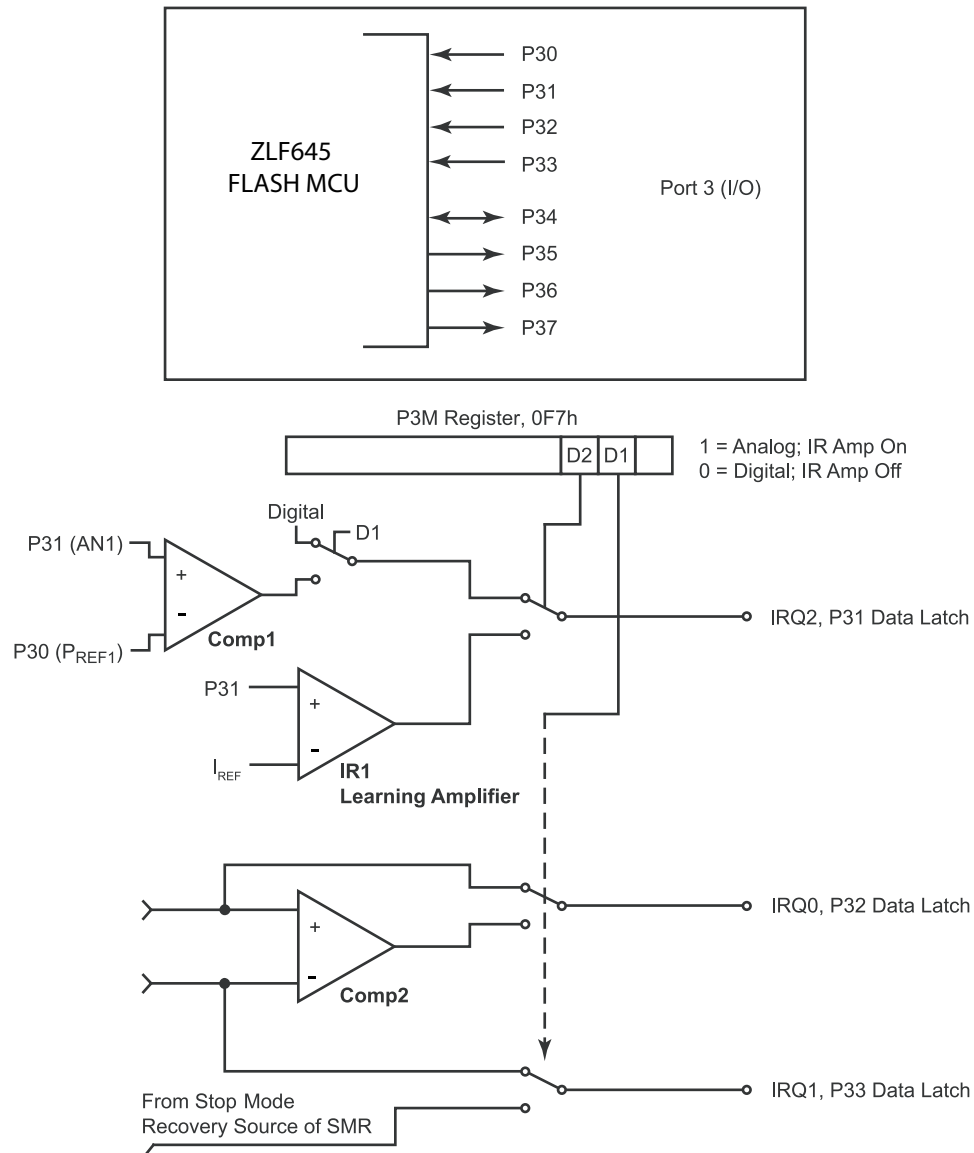
Figure 9. Port 3 Configuration
