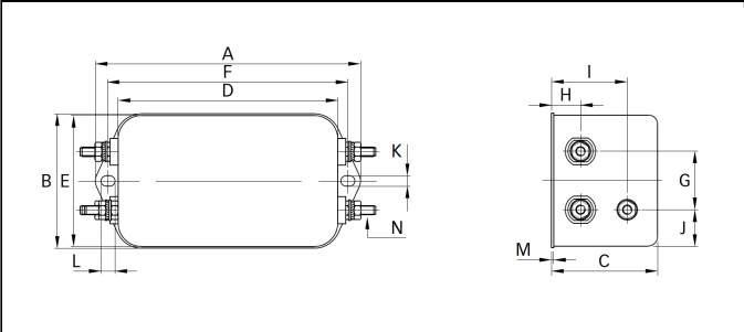
Connection style -08, 20 and 30 A types
