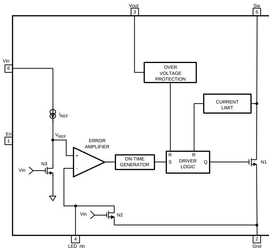
Figure 2. Block Diagram
