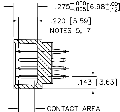
SECTION X-X
