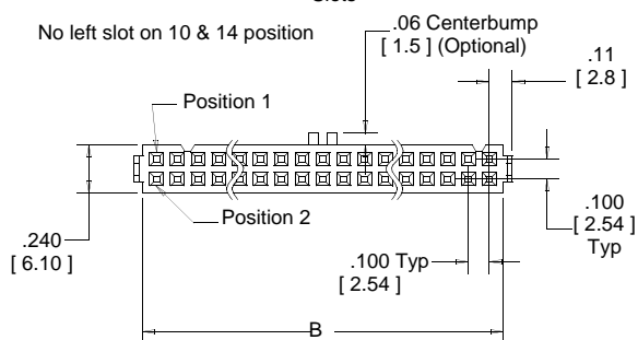
Bottom View of Body
