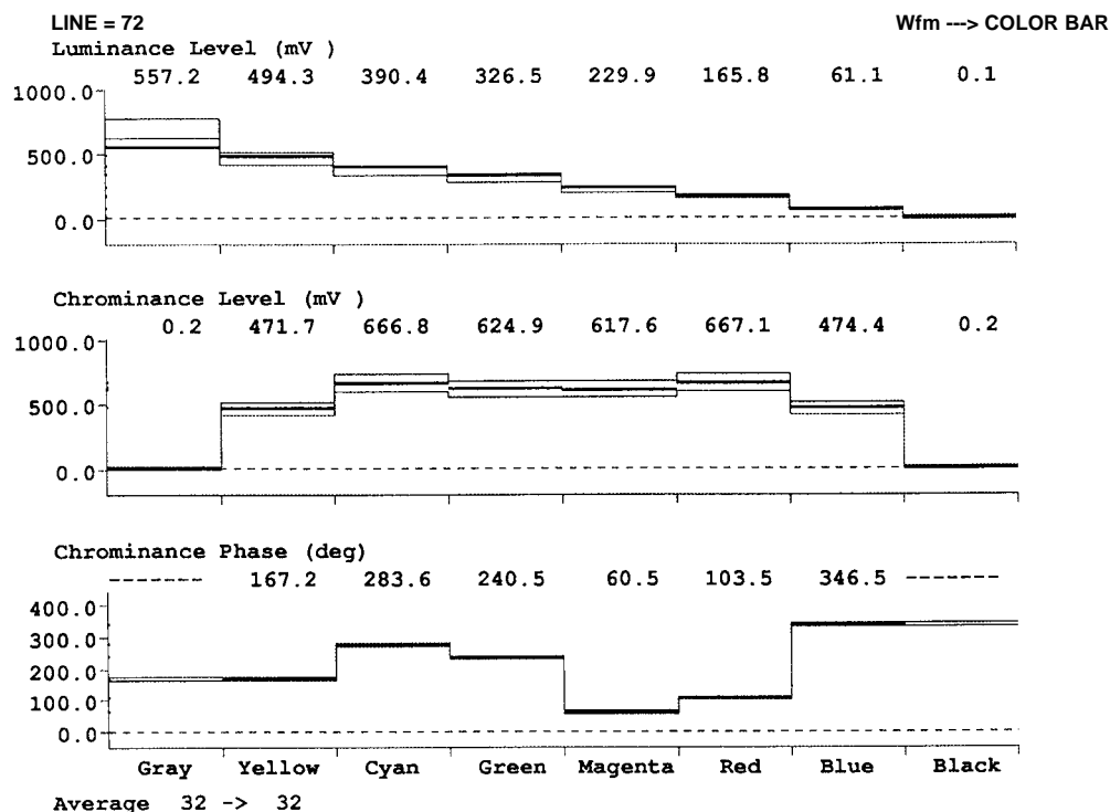
FIGURE 31. COLORBAR (PAL)
