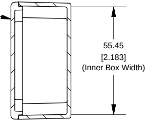
SECTION A-A End View of Assembly
