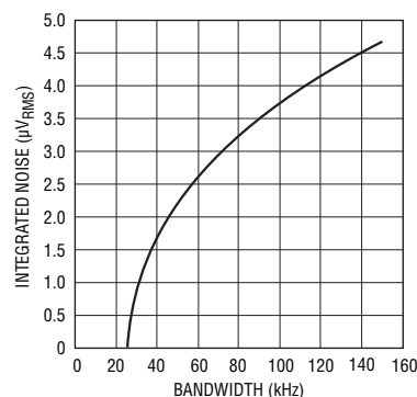
Line Receiver Integrated Noise 25kHz to 150kHz
