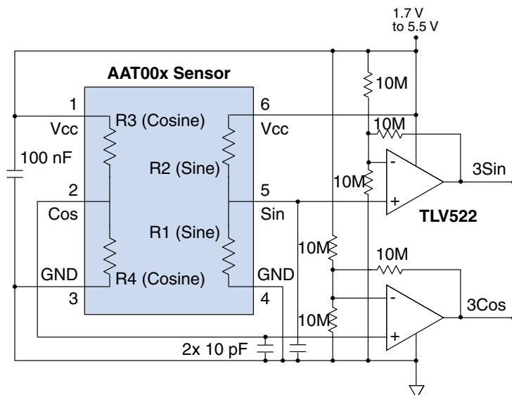
Figure 6. 3x Preamplifier.
