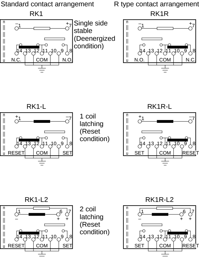
Schematic (Bottom view)
