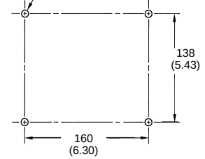
Mounting Holes
