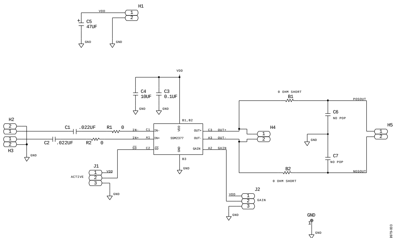
Figure 3. Schematic of the SSM2377 Evaluation Board
