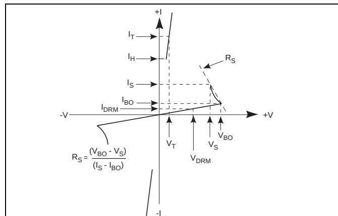
V-I Characteristics
