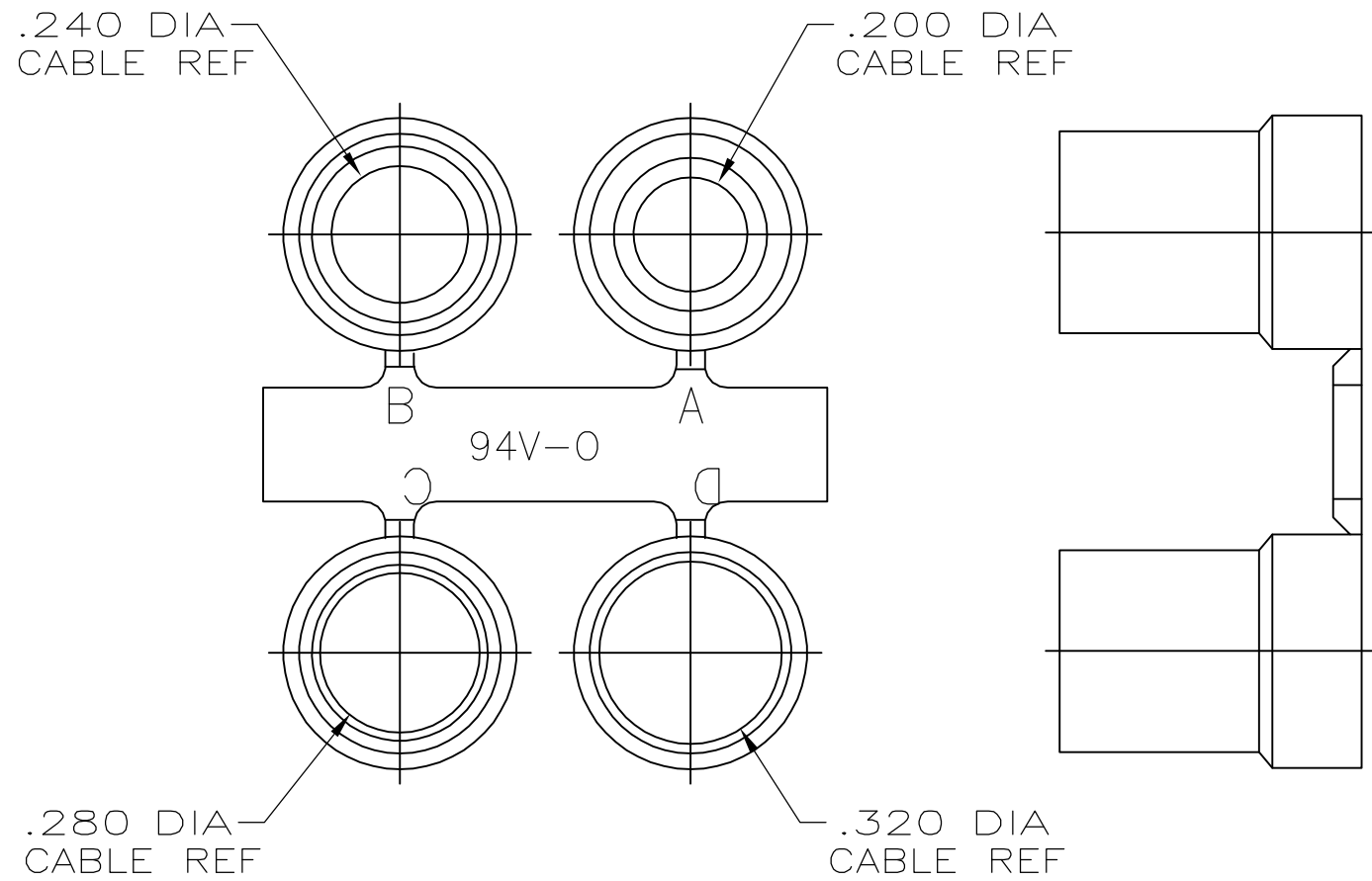
GROMMET ASSORTMENT TYPE 1 SEE TABLE
