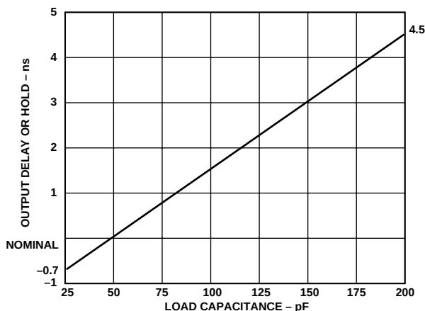
Figure 32. Typical Output Delay or Hold vs. Load Capacitance (at Maximum Case Temperature) ( V_{DD} = 5 \text{ V} )
