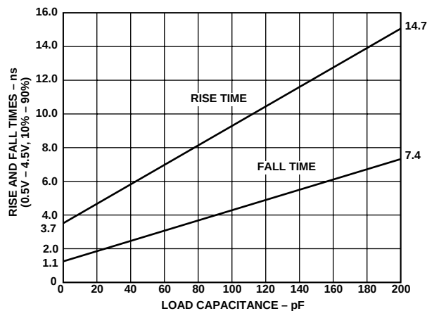
Figure 30. Typical Output Rise Time (10%–90% V_{DD} ) vs. Load Capacitance ( V_{DD} = 5 \text{ V} )
