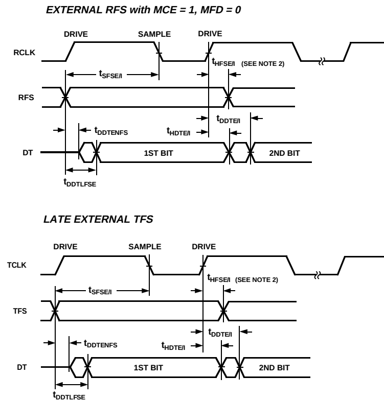
Figure 23. External Late Frame Sync
