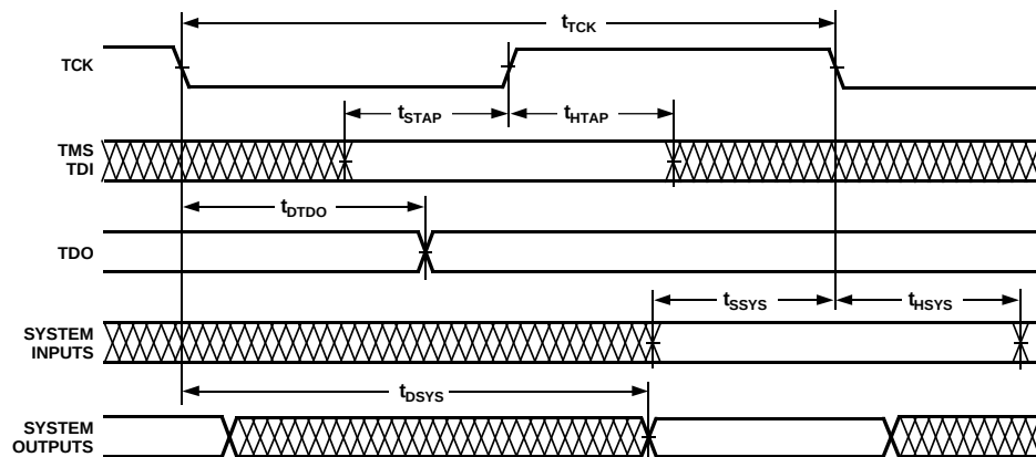
Figure 25. IEEE 1149.1 JTAG Test Access Port
