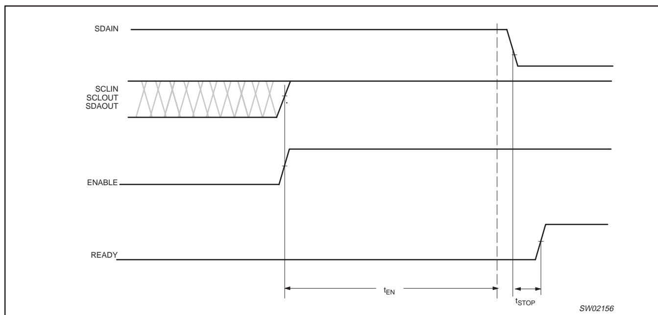
Figure 17. t_{\text{STOP}} that can occur after t_{\text{ENABLE}}
