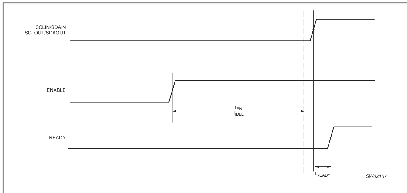
Figure 18. t_{READY} delay that can occur after t_{ENALBE} and t_{IDLE}
