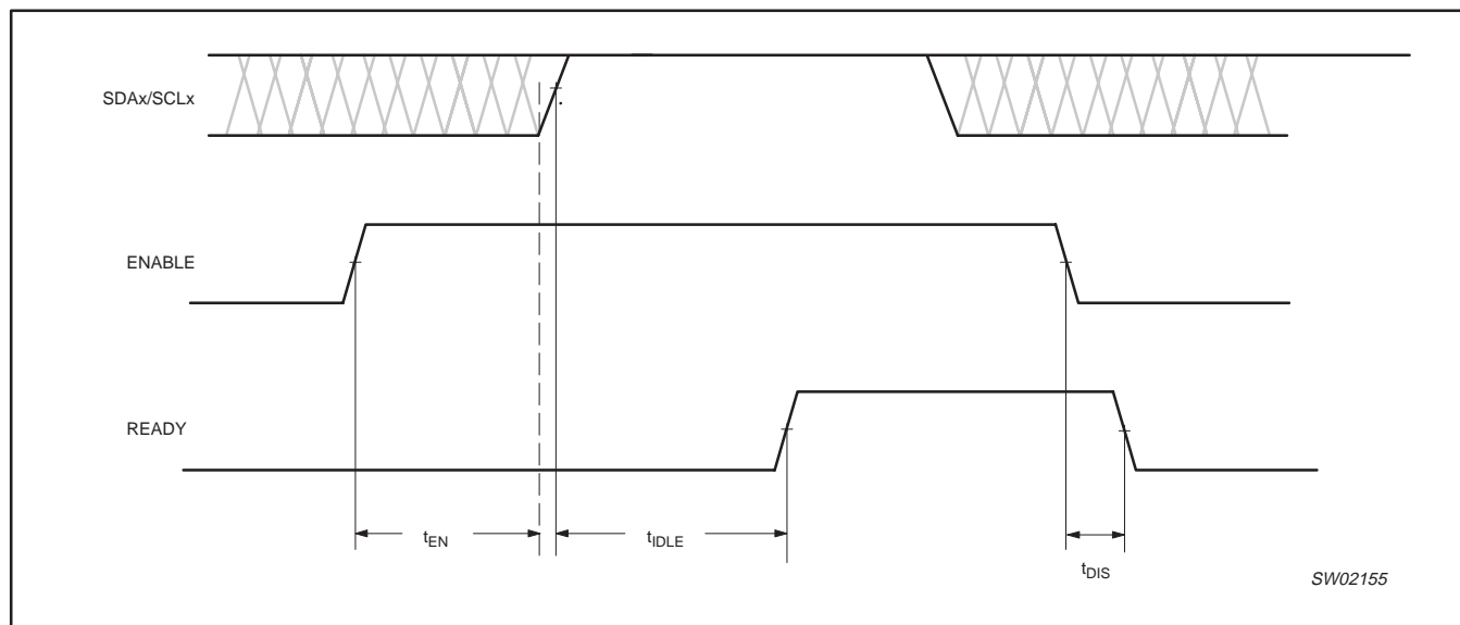
Figure 16. Timing for t_{\text{ENABLE}} , t_{\text{IDLE}} , and t_{\text{DISABLE}}
