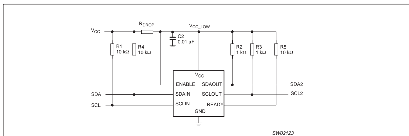
Figure 11. System with disparate V CC voltages
