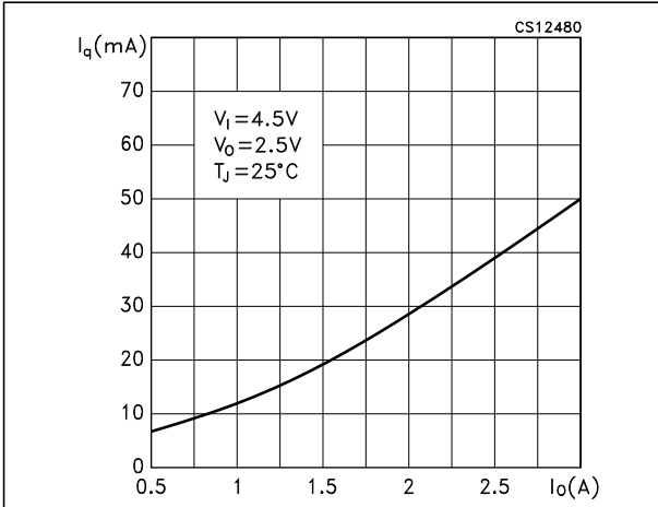
Figure 8. Quiescent current vs. output current ( V_I = 4.5\text{ V} )
