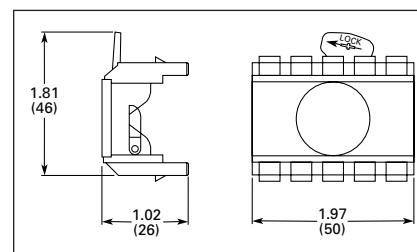
Figure 47-18. Overall Dimensions in Inches (mm)
