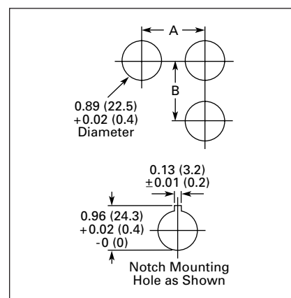
Figure 47-17. Minimum Spacing in Inches (mm)
