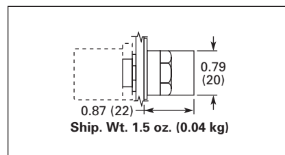
Figure 47-72. EM22 Series — 60° Throw — Knob
