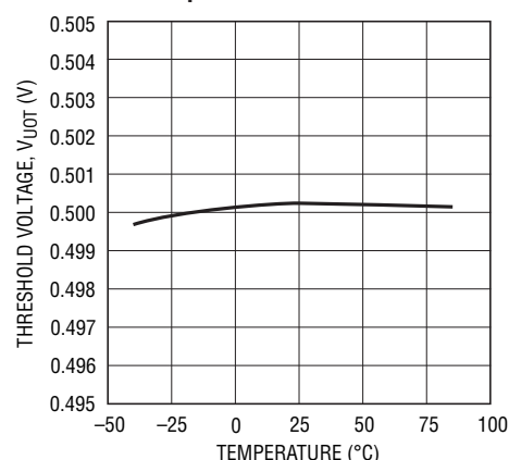
Input Threshold Voltage vs Temperature
