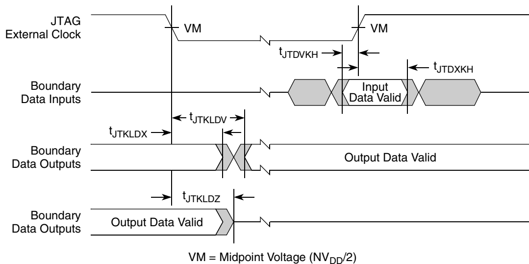
Figure 43. Boundary-Scan Timing Diagram
