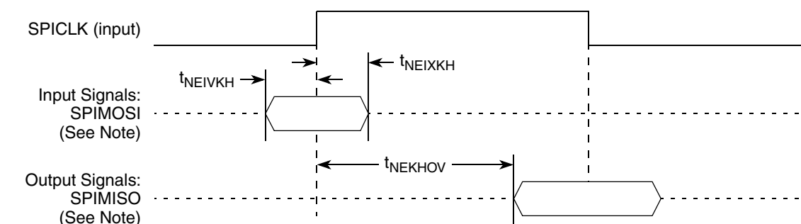
Figure 50. SPI AC Timing in Slave Mode (External Clock) Diagram
