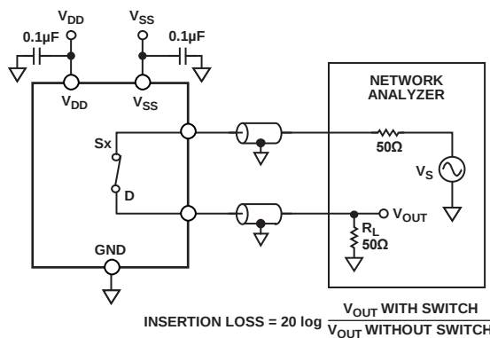
Figure 30. Bandwidth
