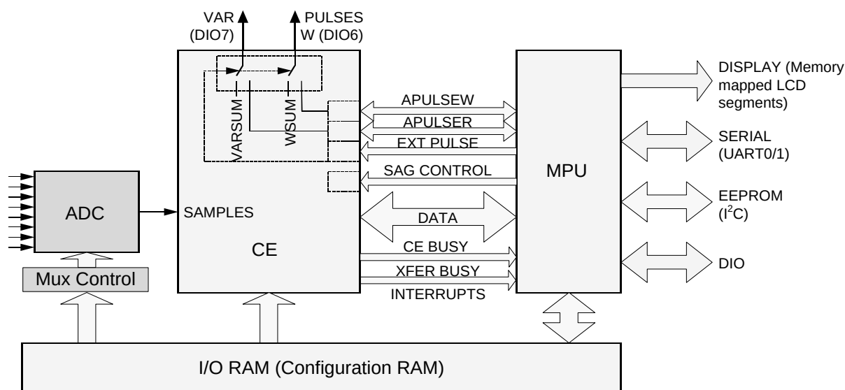
Figure 27: MPU/CE Communication
