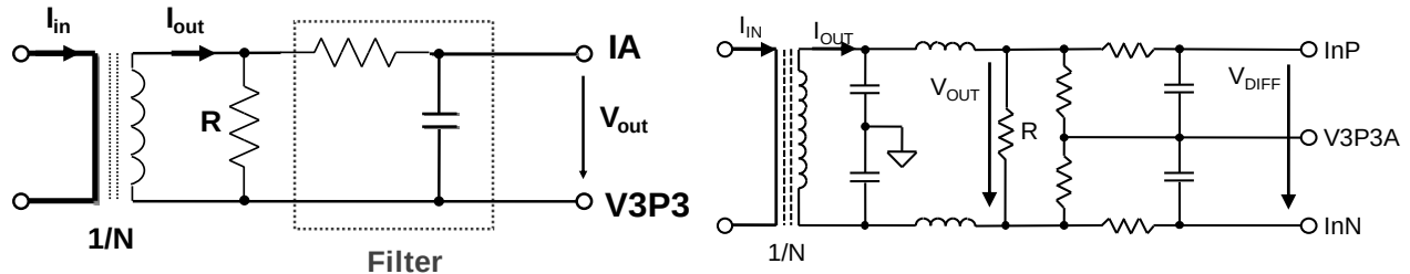
Figure 29: CT with Single Ended (Left) and Differential Input (Right) Connection
