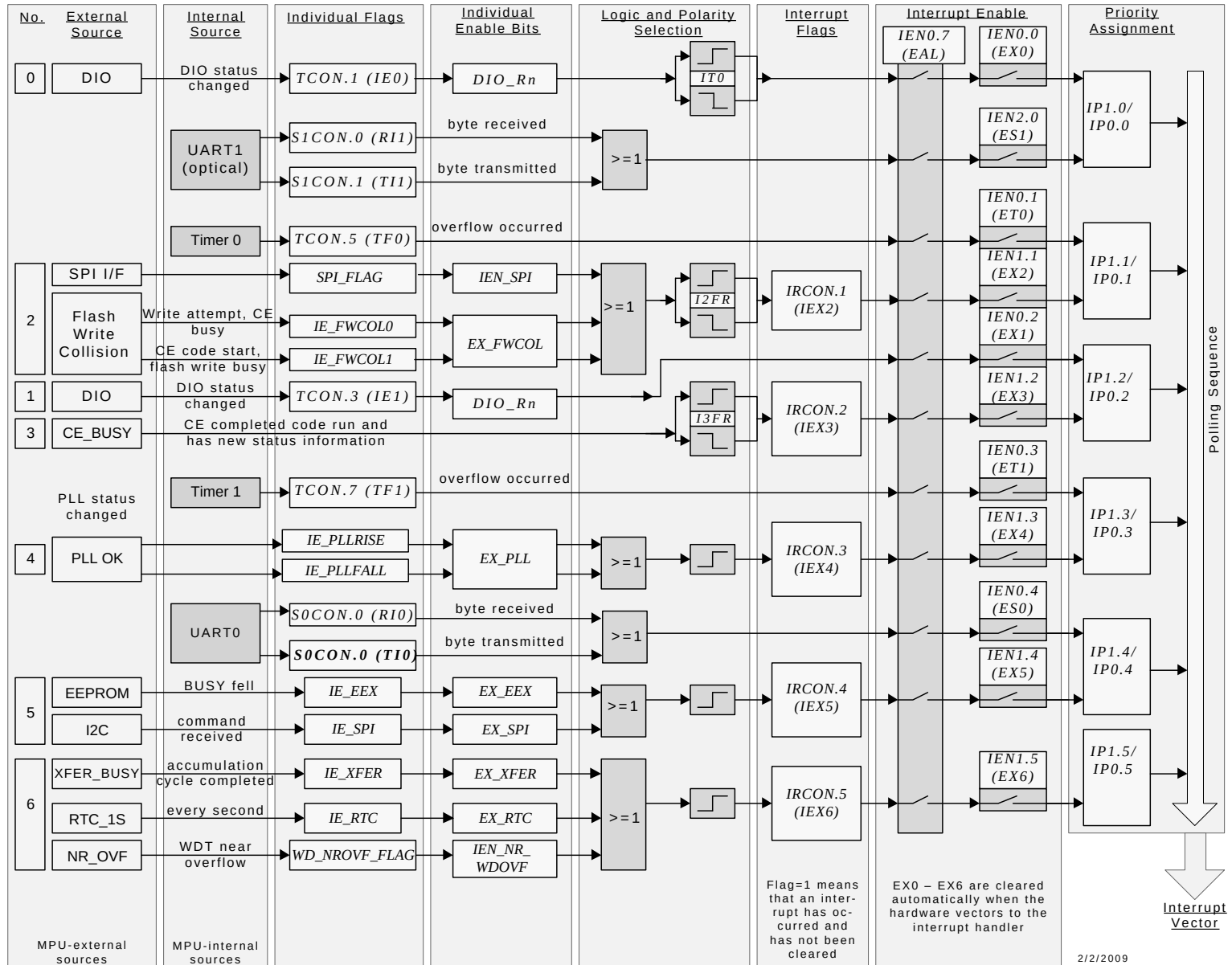
Figure 8: Interrupt Structure
