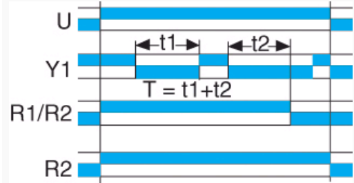
Delay on energisation with memory 2 timers or 2 relays, including 1 instantaneous
