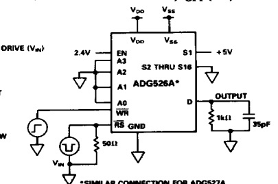
TEST CIRCUIT 10 RESET TURN-OFF TIME, t_{OFF} (RS)
