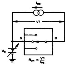
TEST CIRCUIT 2 I_S (OFF)
