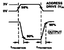
TEST CIRCUIT 6 SWITCHING TIME OF MULTIPLEXER, t_{TRANSITION}
