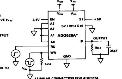
TEST CIRCUIT 10 RESET TURN-OFF TIME, t_{OFF} (RS)
