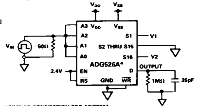
TEST CIRCUIT 7 BREAK-BEFORE-MAKE DELAY, t_{OPEN}
