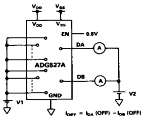
TEST CIRCUIT 5 I_{DIFF}
