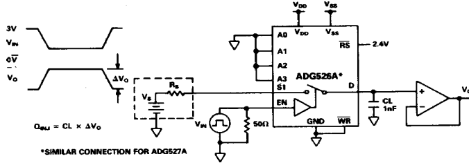
TEST CIRCUIT 11 CHARGE INJECTION
