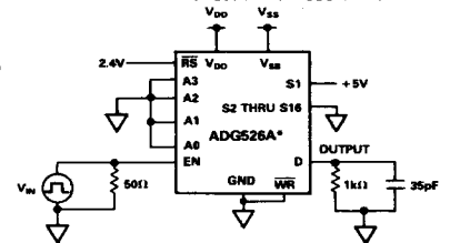
TEST CIRCUIT 9 WRITE TURN-ON TIME, t_{ON} (WR)
