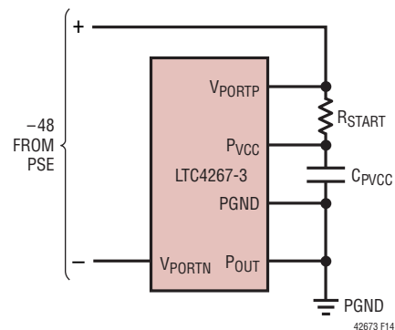
Figure 12. Powering the LTC4267-3 Switching Regulator via the Shunt Regulator
