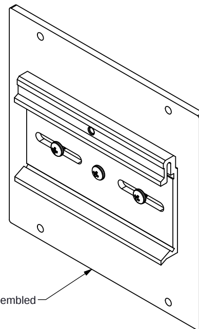
ASSEMBLY VIEW
