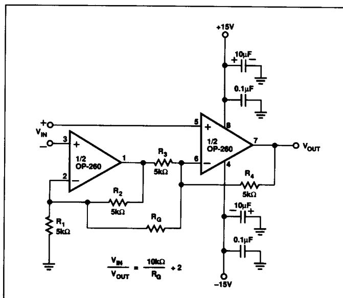
FIGURE 16: High Speed Instrumentation Amplifier
