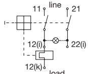
2-pole, unprotected
