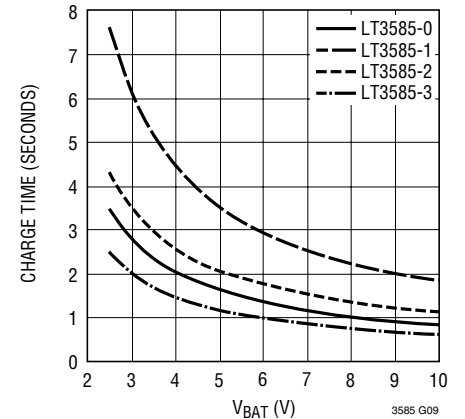
Charge Time* Normal Input Current Mode
