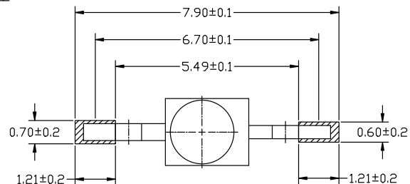
RECOMMENDED MOUNTING FOOTPRINT
