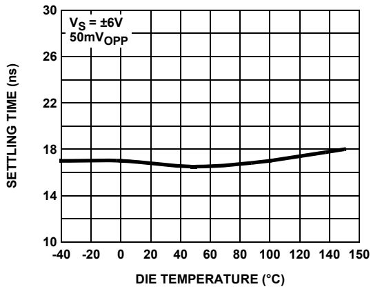
FIGURE 39. 0.1% SETTLE TIME vs TEMPERATURE
