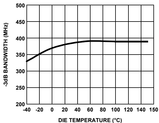
FIGURE 37. -3dB BANDWIDTH vs TEMPERATURE
