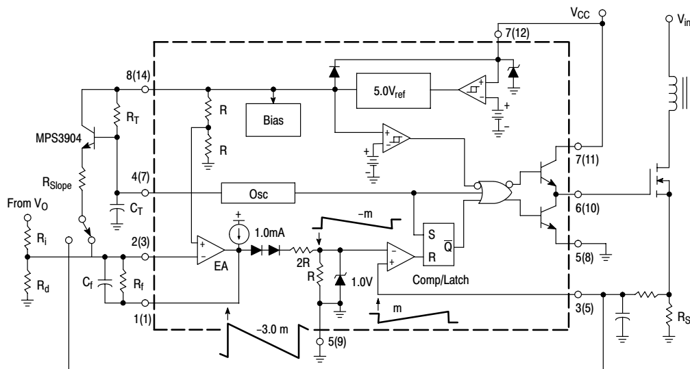
Figure 33. Slope Compensation
