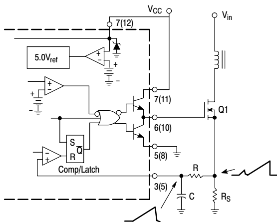
Figure 27. Current Waveform Spike Suppression
