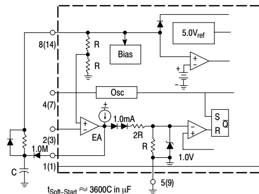
Figure 24. Soft-Start Circuit
