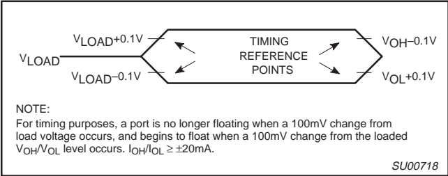
Figure 48. Float Waveform
