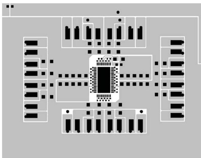
Figure 4. PCB Layer 1
