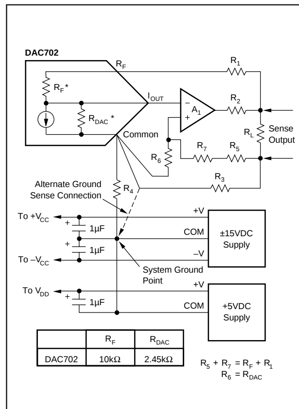
FIGURE 8. Differential Sensing Output Op Amp Configuration.
