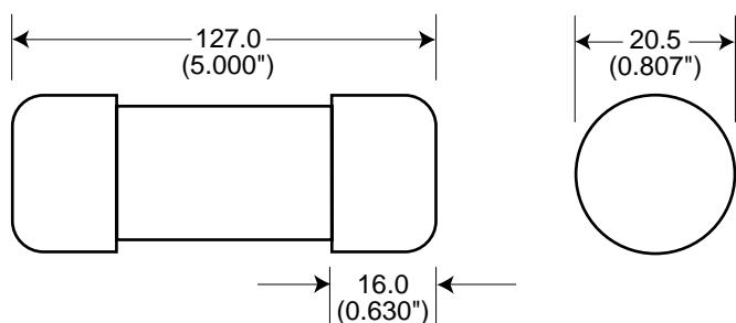
Fig. 2: 35-60 Amp Range
