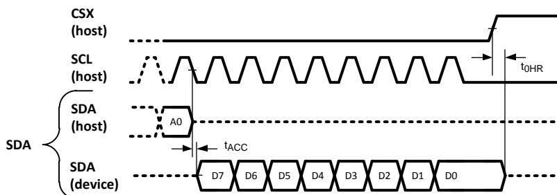
Figure 5. SPI Interface
