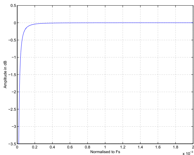
Figure 9-5. DAC HPF Response
