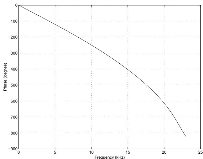
Figure 9-9. Phase Response—ADC, Notch Disabled
