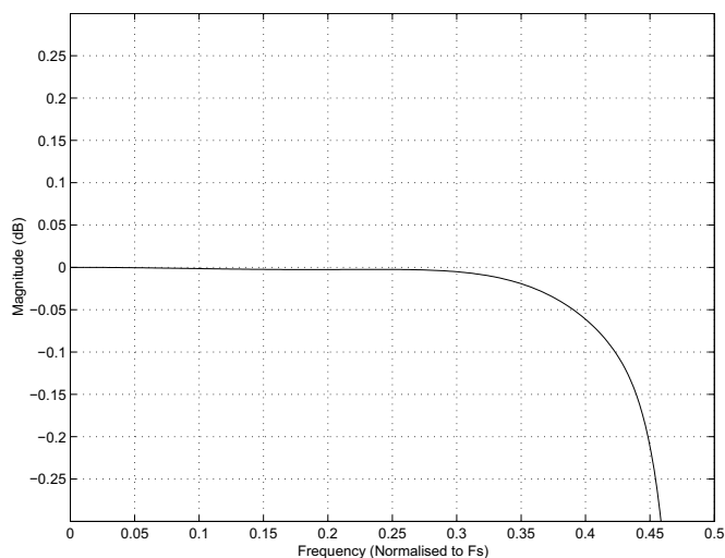
Figure 9-6. Passband—ADC, Notch Disabled
