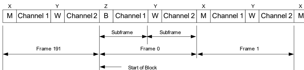
Figure 4-39. S/PDIF Frame Format
