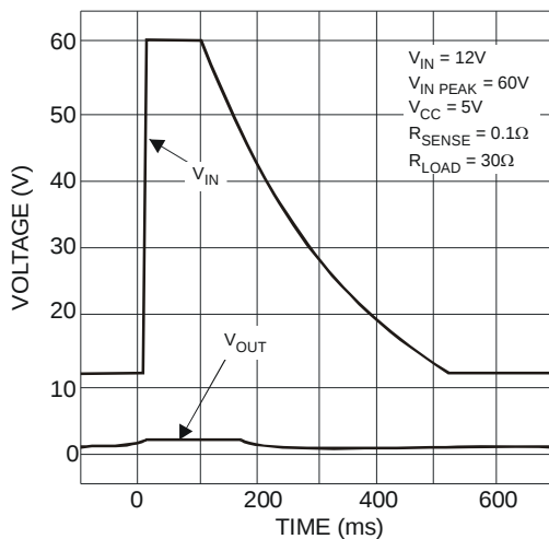
Fig. 16 Load Dump Waveform
