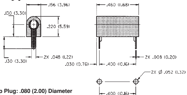
MOUNTING HOLE LAYOUT
