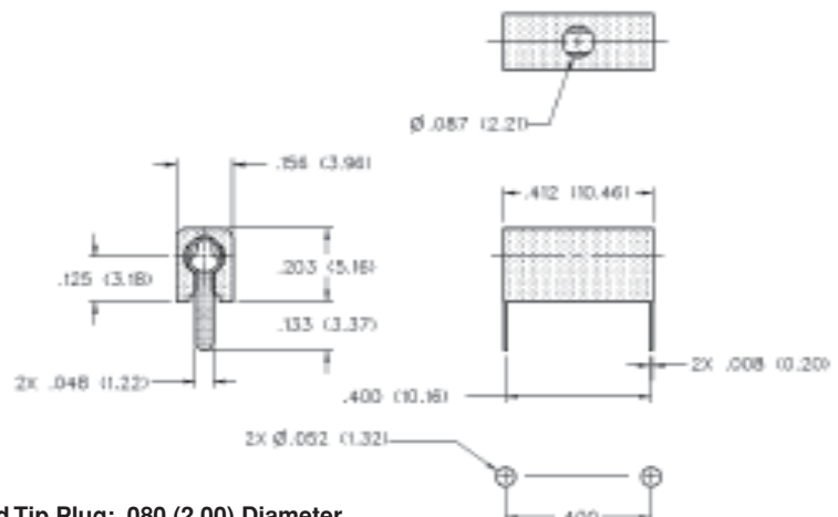
MOUNTING HOLE LAYOUT
