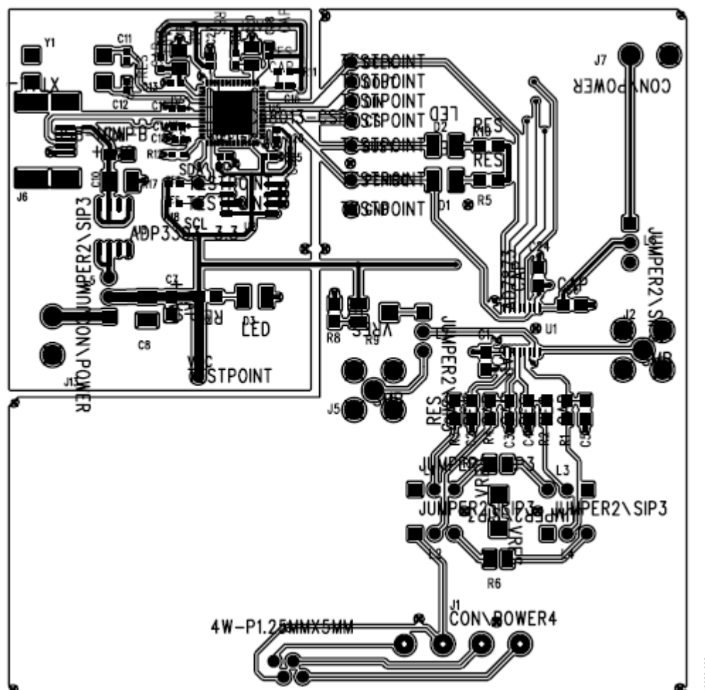
Figure 8. AD7843AD7873 Evaluation Board Component Side
