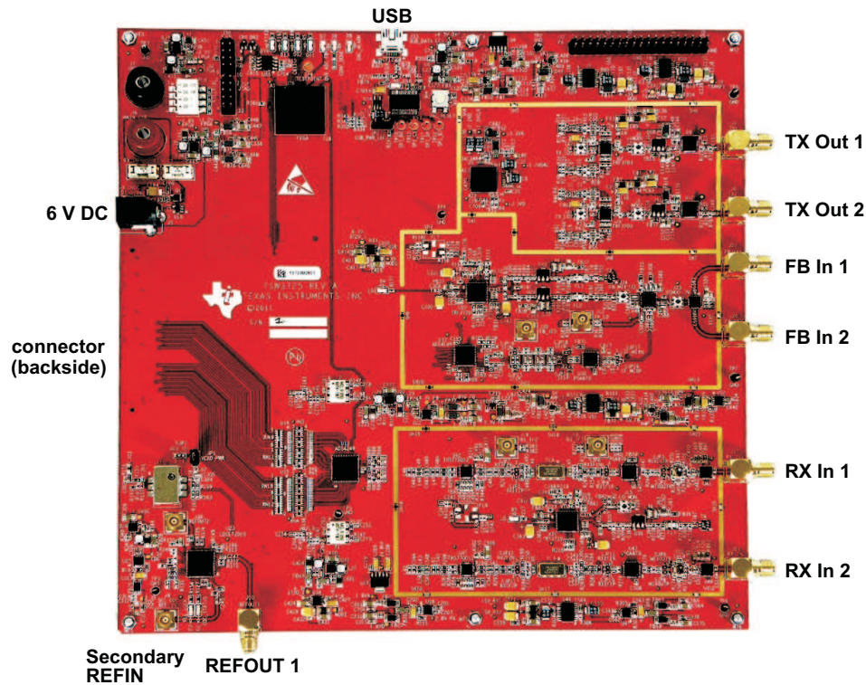
Figure 2. TSW3725EVM
