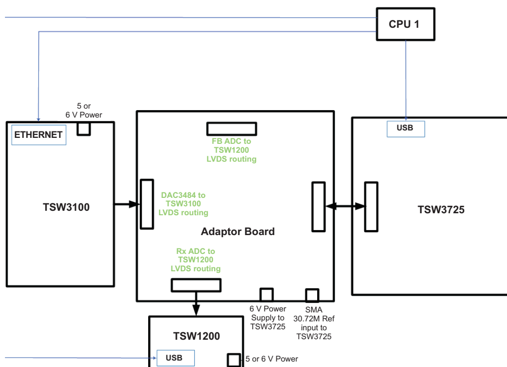
Figure 6. 2 TX and 2 RX Configuration
