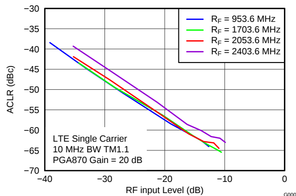
Figure 69. FB ACLR vs Input Amplitude/Frequency LTE 10 MHz TM1.1
