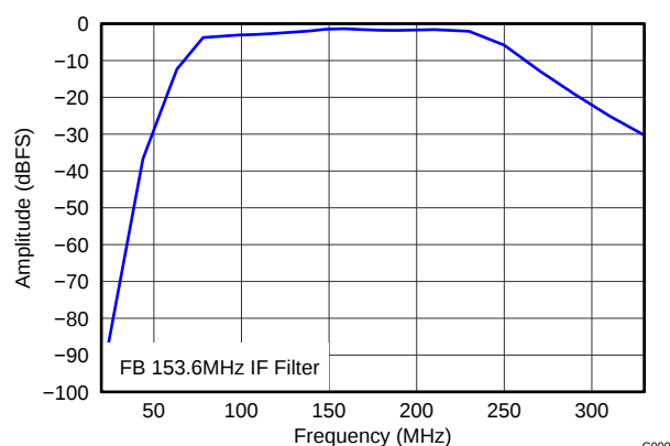
Figure 71. FB IF Filter Response
