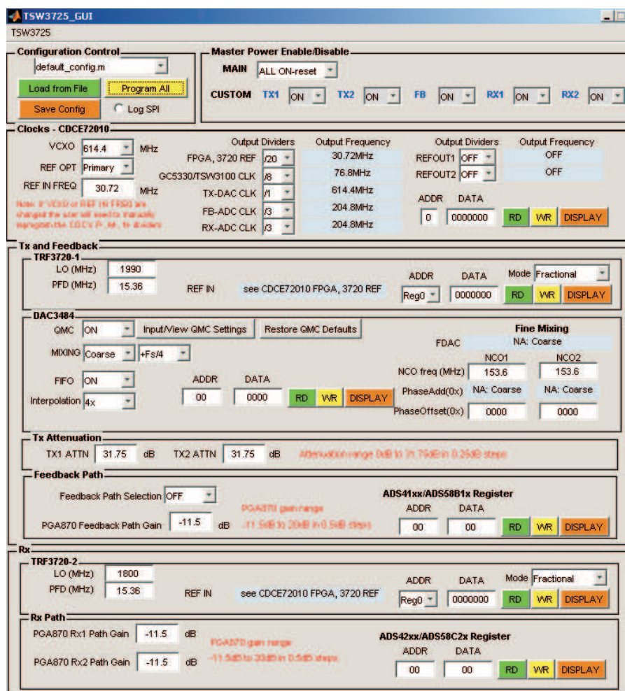
Figure 27. TSW3725 GUI
