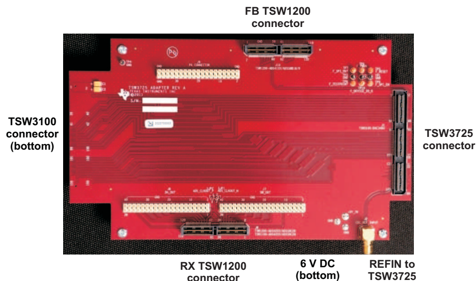
Figure 3. TSW3725 Rev-A Adaptor
