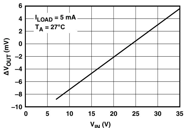
Figure 9. Line Regulation
