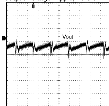
Output Voltage Ripple, Version B (4.5V)
