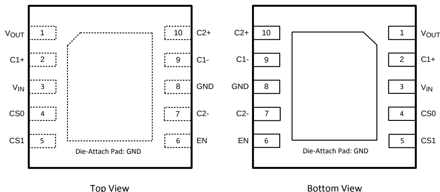
Figure 1. 10-pin SON No Pullback Package (3mm × 3mm × 0.8mm) See Package Number DSC0010A
