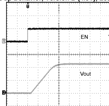
Start-up Behavior, Version B (4.5V), Load = 150mA
