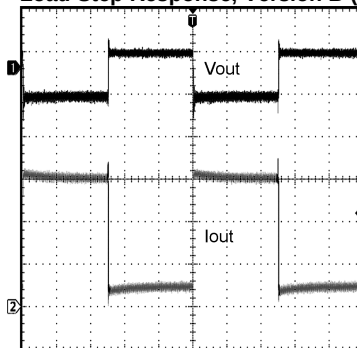
Load Step Response, Version B (4.5V)
